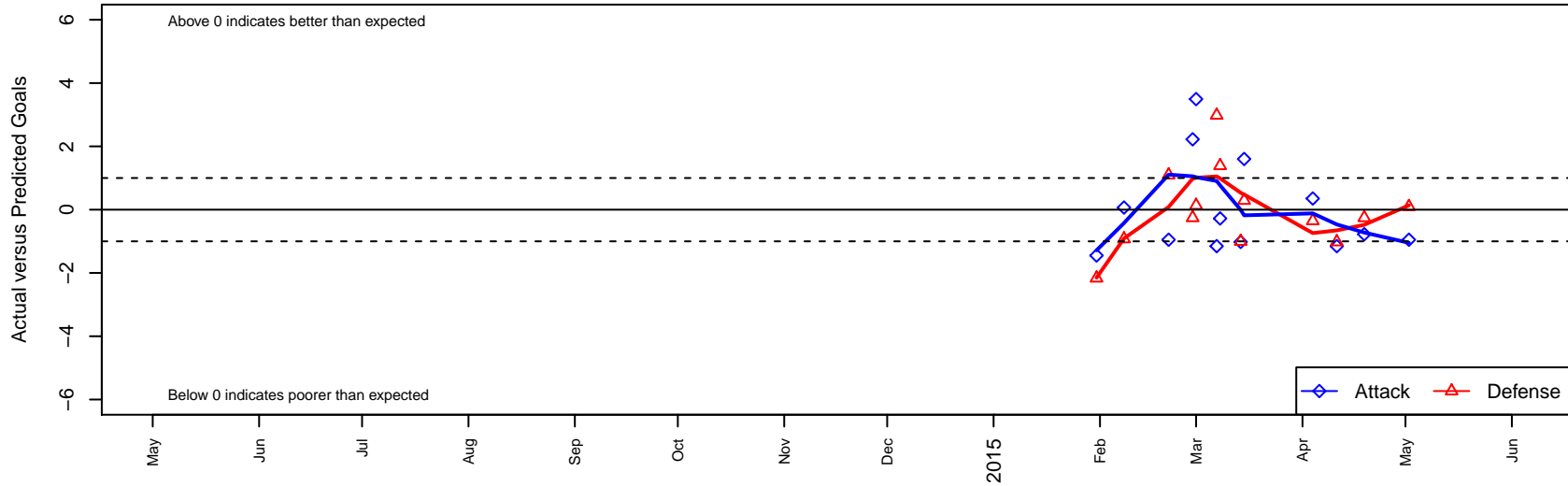
BSC Hood River Venom G99 Dots are actual minus expected GF (blue circles) and GA (red triangles). Blue line is smoothed change in attack strength. Red is smoothed change in defense strength.
